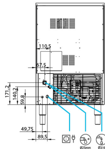
REAR VIEW
