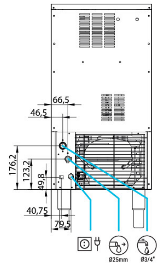
REAR VIEW
